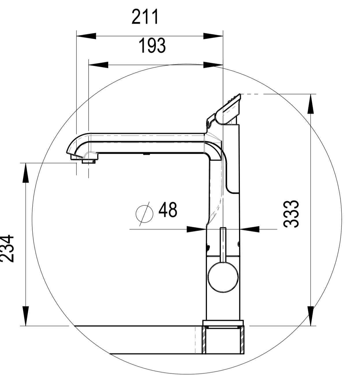
DETAIL FONT SCALE 1 : 4
